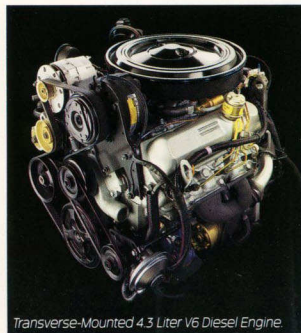
Transverse-Mounted 4.3 Liter V6 Diesel Engine.
