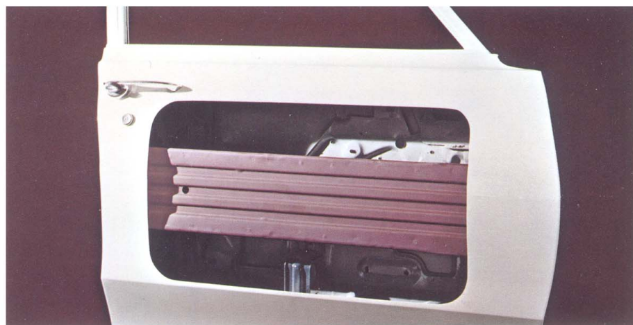
Side-guard Door Beam. Every side door in every '70 Pontiac has a sturdy, reinforced steel beam built in for added security. All 4-door models also have reinforced center pillars. Only one example of the added security from Pontiac.
