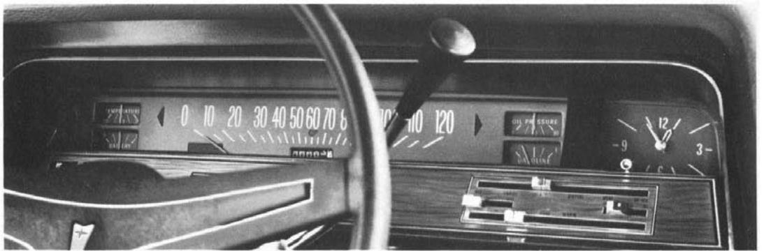
Custom Gauge Cluster (Code 484—UPC W63). This option groups water temperature gauge and ammeter together, and fuel and oil pressure gauges together on Catalina, Executive and Bonneville and includes clock and speedometer, where not already standard. Illustrated is Custom Gauge Cluster with clock on Executive model. (F)
