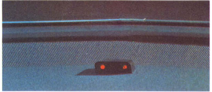
Monitoring System for Rear Lamps. (Code 634—UPC U46). New and available all series. Uses plastic fibers to transmit light from rear lamps to indicator on back window shelf, thus verifying that lamps are working. All models except station wagons and convertibles. (F,D)
