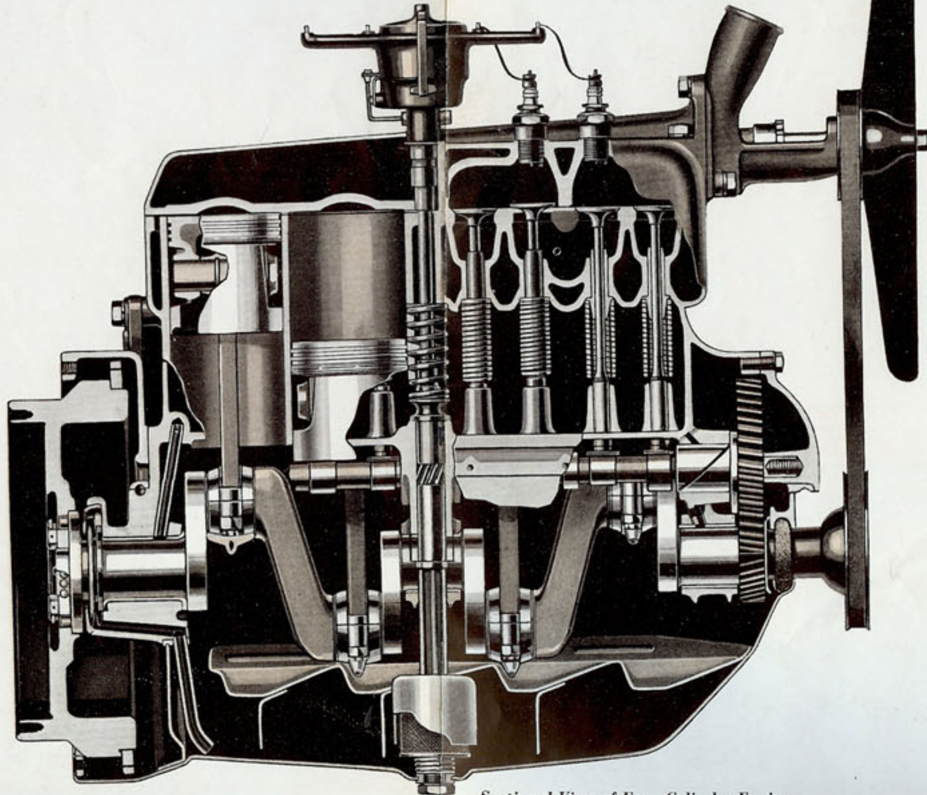
Sectional View of Four Cylinder Engine
